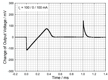
Abb. 16. Transient load regulation of the negative output voltage at 100% load change.
